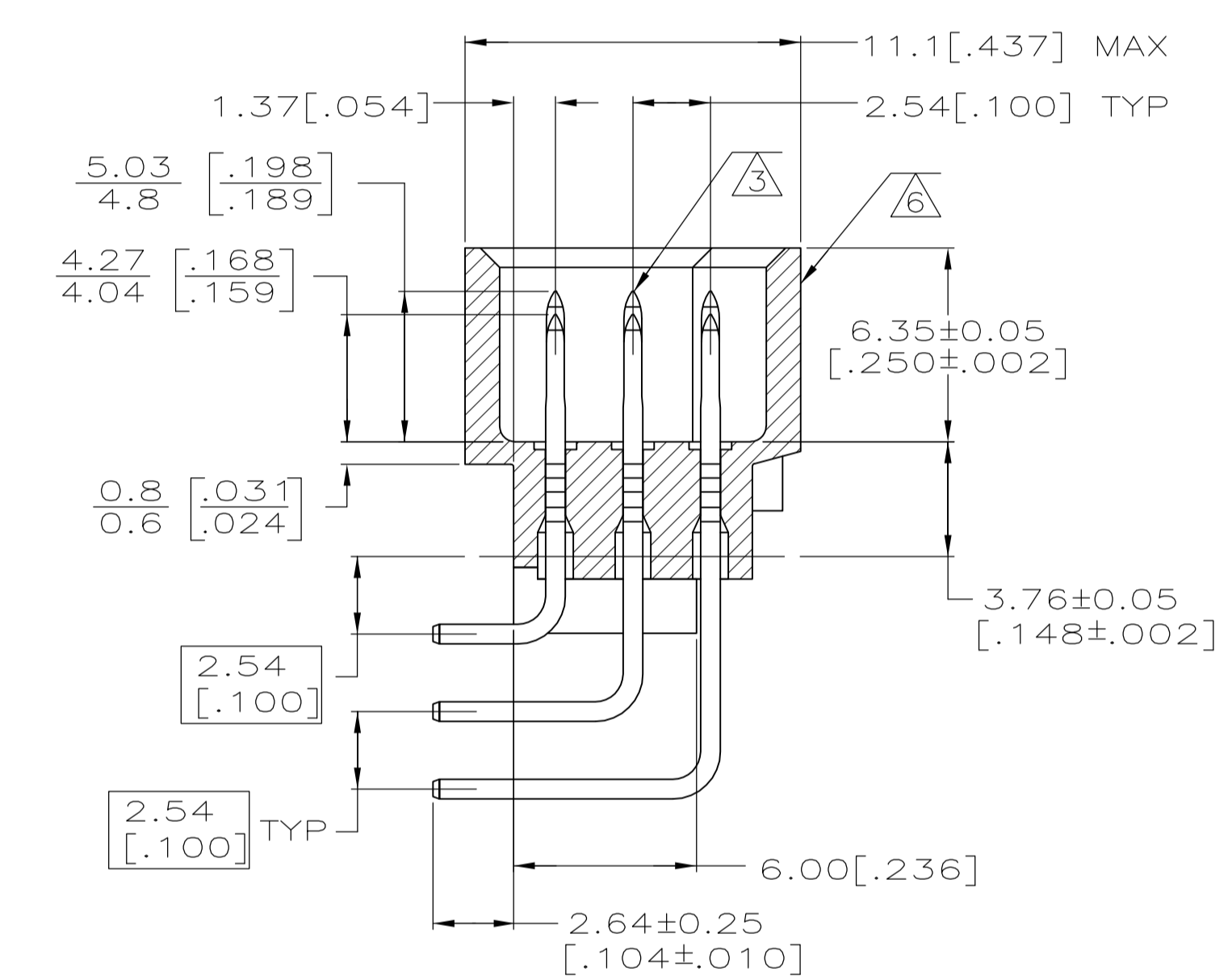
SECTION Z-Z
